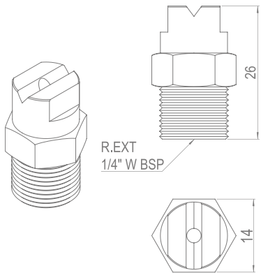
FOG NARROW NOZZLE
