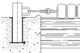
Anchor code 00141 Lane rope support code 00140
