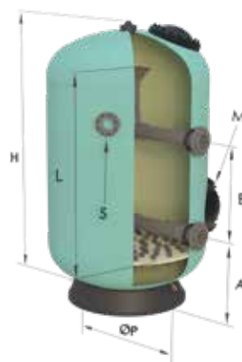
Filter with nozzle plate
