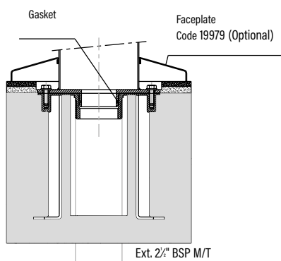
Anchor detail
