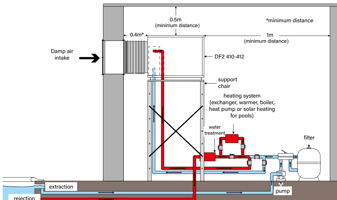
Example of an installation with a DF2
