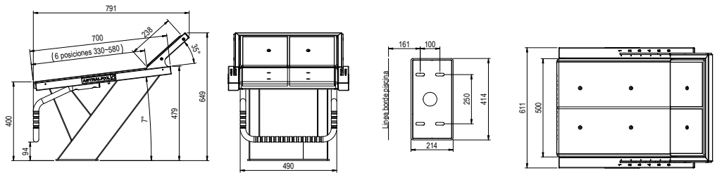
Competition starting block
