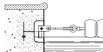
Anchoring cup code 09206 code 09207 code 00205 code 00206
