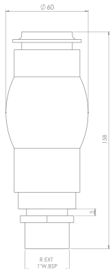
FOAMY NOZZLE 32 PL/SS
