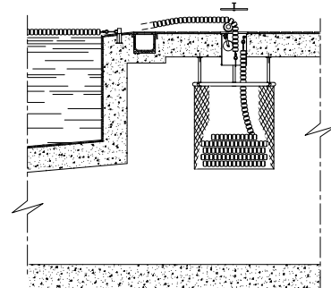
Standard type Installation diagram
