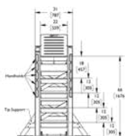
168 cm Sentry Lifeguard chair with center supports
